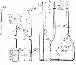
Figs. 4895-96. PEDESTAL BRAKE-BEAM TIE-BAR SAFETY-STAY-ROD. Figs. 4897-98. HANGER.
